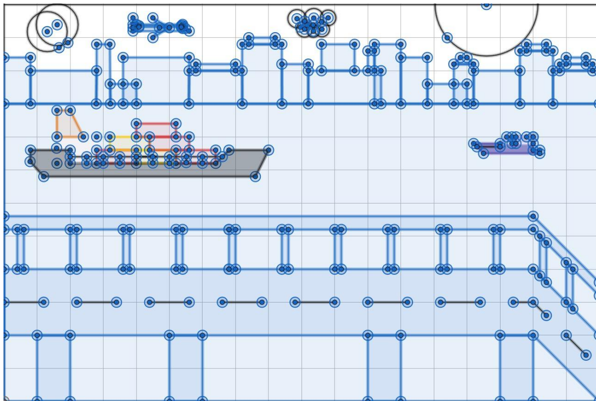
Figure 1: Scene 3 (Bridge) plotted on Geogebra [No labels]
