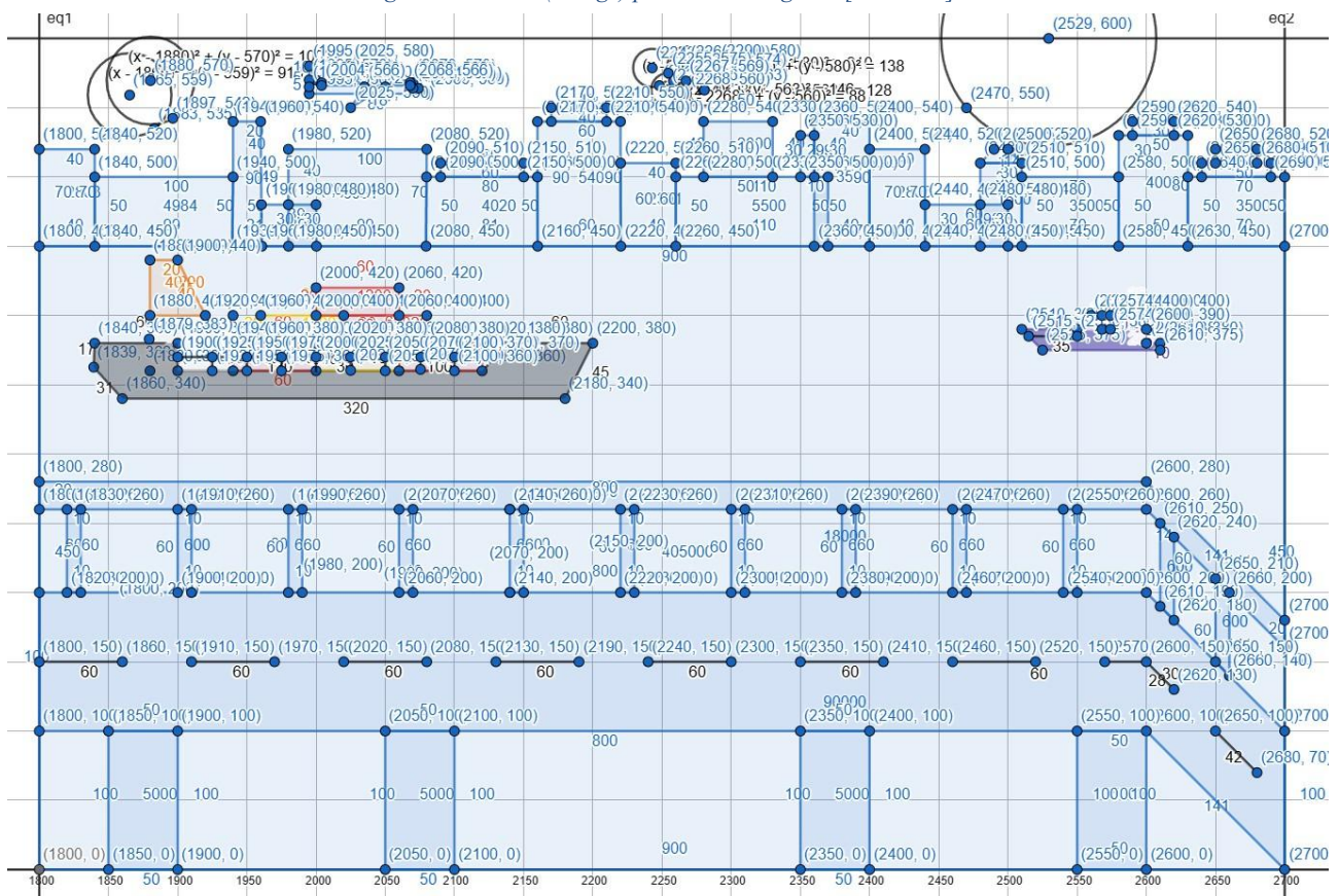
Figure 2: Scene 3 (Bridge) plotted on Geogebra [With labels]
